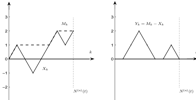
Fig. 6.3. On the left an embedded random walk \{X_k : k \geq 0\} together with its maximum process \{M_k : k \geq 0\} . On the right the associated difference process \{Y_k : k \geq 0\} defined by Y_k = M_k - X_k .
