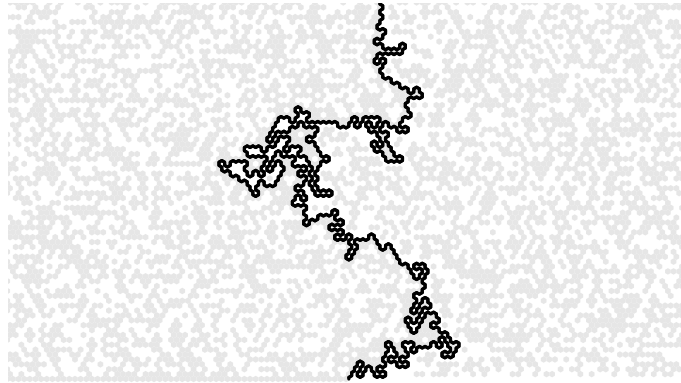
Fig. 11.7. Beginning of the percolation interface in the upper half-plane
