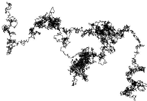
Fig. 0.1. The range of a planar Brownian motion \{B(t) : 0 \leq t \leq 1\} .
