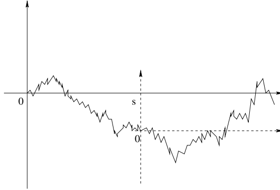
Fig. 2.1. Brownian motion starts afresh at time s .
