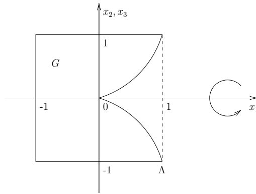
Fig. 8.2. Lebesgue's thorn.
