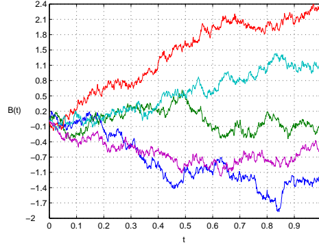
Fig. 1.1. Graphs of five sampled Brownian motions
