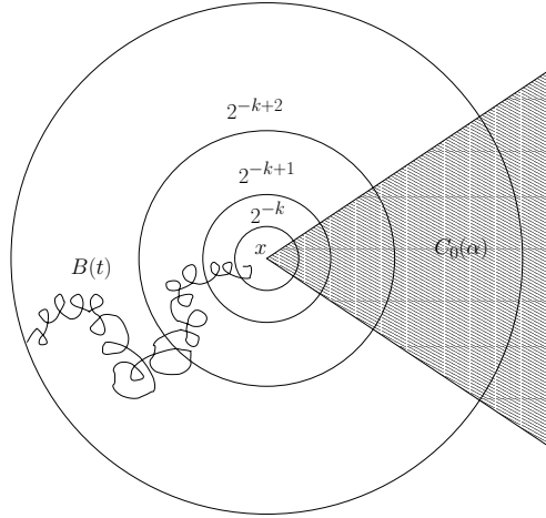
Fig. 3.1. Brownian motion avoiding a cone.
